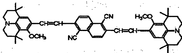
Structural formula (17)-5:
